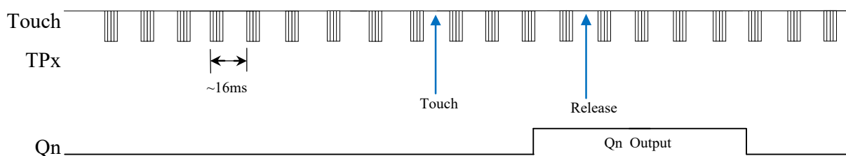
Normal working mode sequence diagram (MLP connected to VDD):
