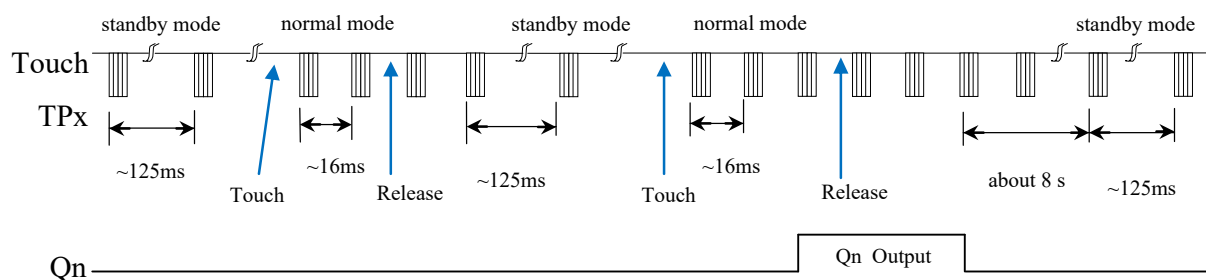
Standby mode timing diagram (MLP left floating or connected to GND) :
