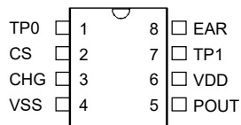
VK36T3D SOP8
