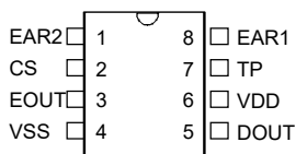
VK36T3A SOP8
