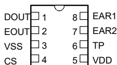
VK36T3A DFN8L
